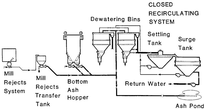
FIGURE C14.6 Single line drawing of sluice system.
