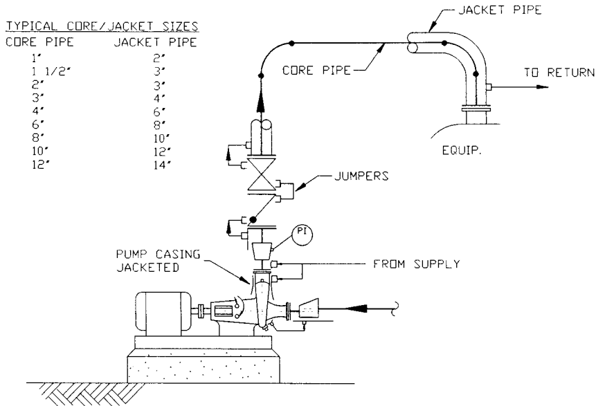
FIGURE C7.12 Jacket liquid phase—circuitry.
