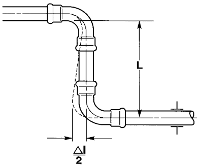
FIGURE A9.5 Z-shaped expansion compensator.
