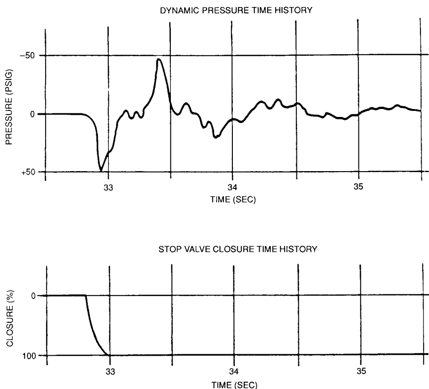
FIGURE B4.13 Steam hammer flow transients.
