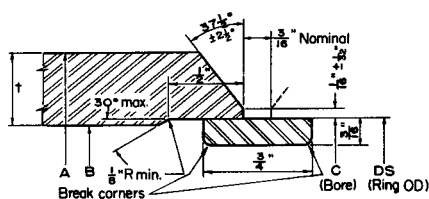
FIGURE A2.23 Typical end preparations for pipe which is to be welded by the inert-gas tungsten-arc welding process.
