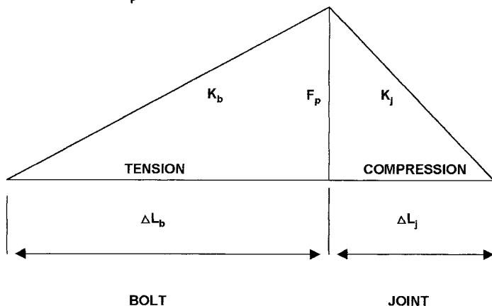
FIGURE A7.12 Joint diagram of simple elastic joints.
