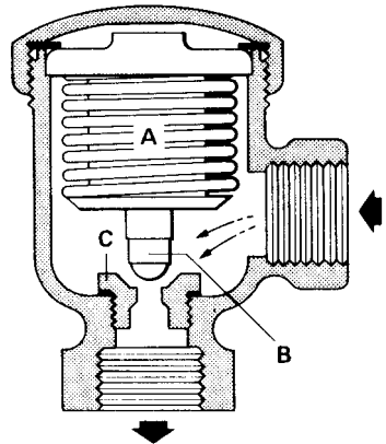
Balanced Pressure Thermostatic Trap
