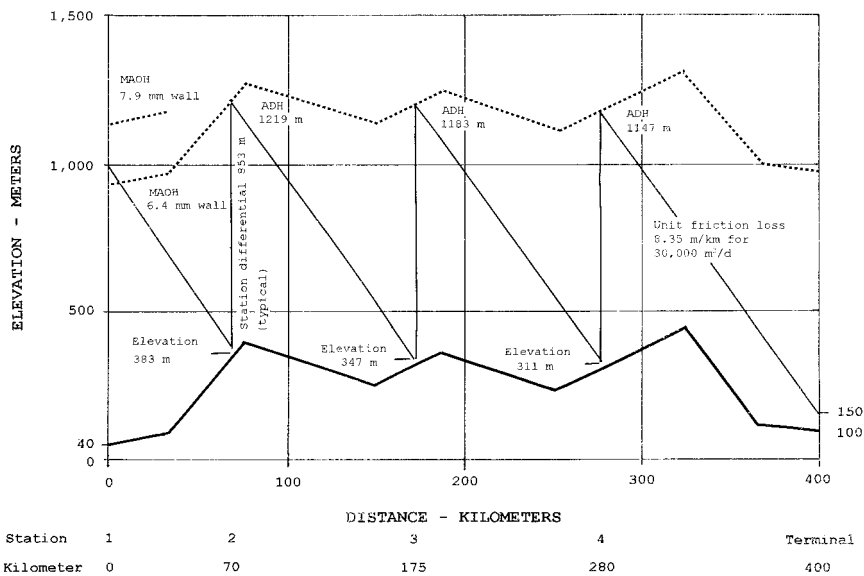
FIGURE C5.8 Hydraulic gradient for DN 500 pipeline example, 30,000 m³/d.
