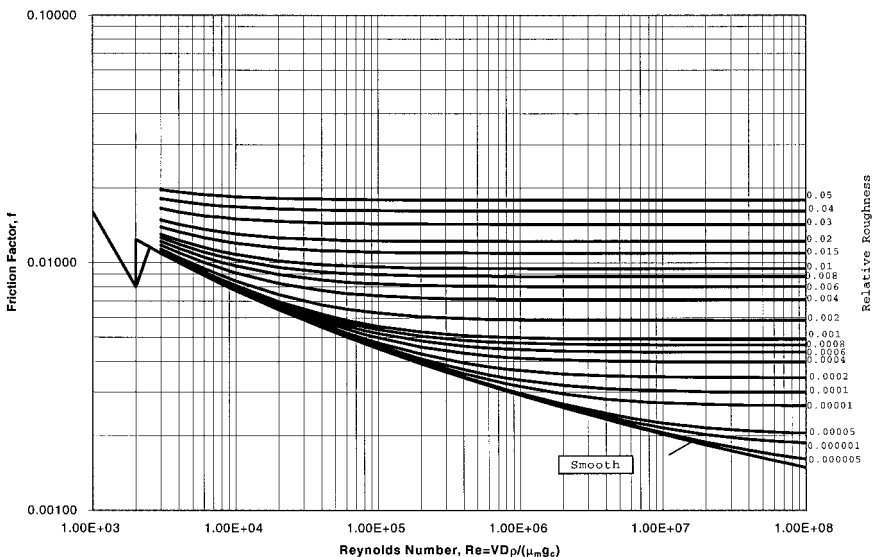
FIGURE C11.6 Friction factor f as a function of Reynolds number for newtonian slurries, where D = pipe ID (ft), V = velocity (ft/s), \rho = density (lb/ft 3 ), \mu = viscosity (lb f ·s/ft 2 ), g_c = 32.2 \text{ lb} \cdot \text{s} / (\text{lb}_f \cdot \text{ft}^2) .
