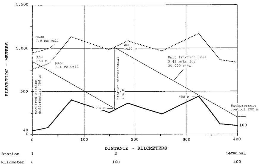
FIGURE C5.9 Hydraulic gradient for DN 600 pipeline example, 30,000 m³/d with profile control point and backpressure control at terminal.
