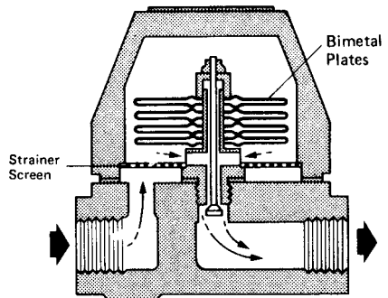
Trap Strainer Unit
