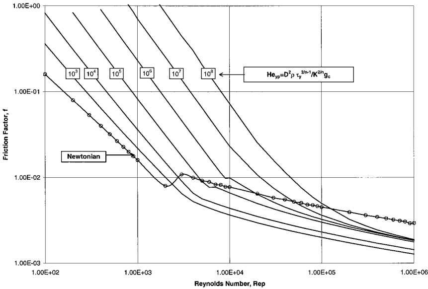
FIGURE C11.9a Friction factor f as a function of Reynolds number for yield pseudoplastic slurries for n = 0.7 , He = [D^2 \rho \tau_y (t_y / K)^{2/n-2}] / (K^2 g_c) , Re = 8 \rho D^n V^{2-n} [n / (2 + 6n)]^n / (K g_c) , where D = pipe ID (ft), V = velocity (ft/s), \rho = density (lb/ft 3 ), K = consistency (lb \cdot s n /ft 2 ), \tau_y = yield stress (lb/ft 2 ), g_c = 32.2 lb \cdot s/(lb \cdot ft 2 ).
