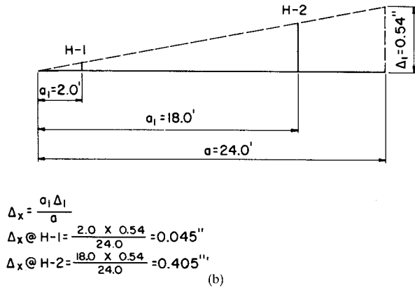
FIGURE B4.26 (a) Deflections of vertical leg of Fig. B4.24. (b) Determination of deflections at H-1 and H-2 of Fig. B4.24.
