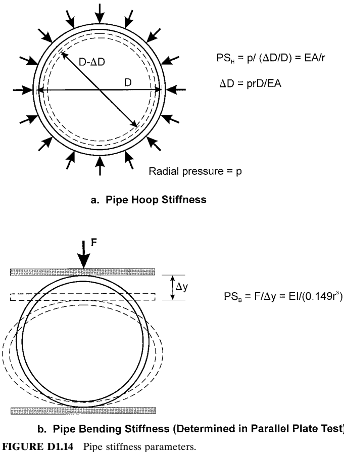
FIGURE D1.14 Pipe stiffness parameters.
