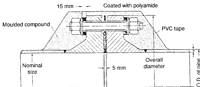
FIGURE C6.19 Insulating flange connection for laying in the ground. (Eisenbau Albert Zieffle KG.)
