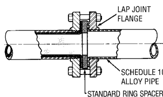
FIGURE B12.4 Recommended installation of plastic-lined pipe to carbon-steel, alloy and non-metallic piping systems. (Courtesy of Crane Resistoflex)
