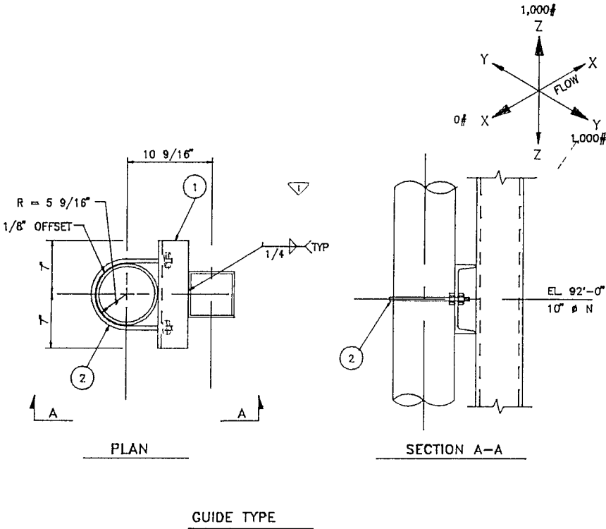
FIGURE C14.19 Sliding pipe support.
