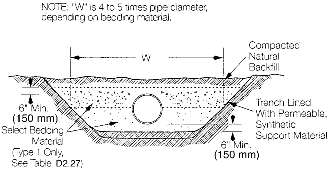
FIGURE D2.17 Wide trench for very soft consistency soils.
