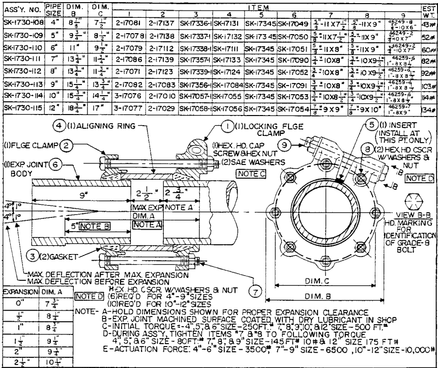
FIGURE C14.17 Cross section of sleeve-type expansion joint (UCC).
