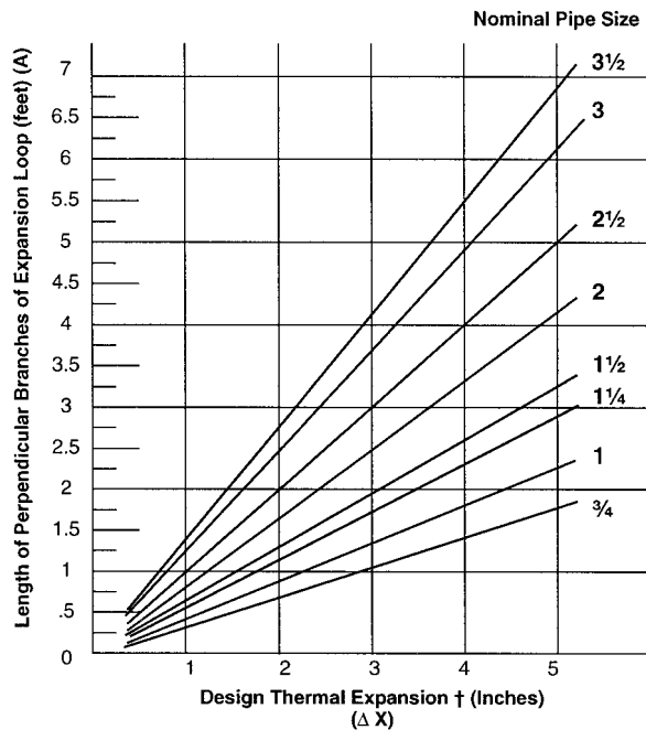
FIGURE A9.22 Expansion loop design.
