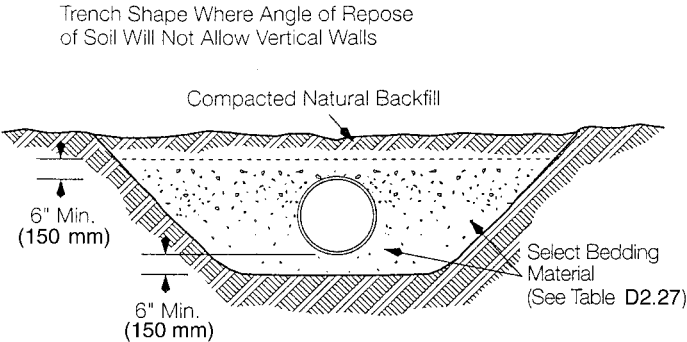
FIGURE D2.16 Trench shape and bedding for granular type soils (sand, etc.).
