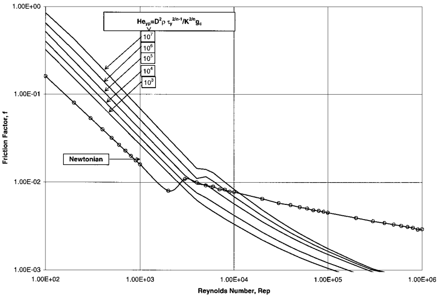
FIGURE C11.9c Friction factor f as a function of Reynolds number for yield pseudoplastic slurries for n = 0.3 , He_p = [D^2 \rho \tau_y (t_y/K)^{2/n-2}] / (K^2 g_c) , Re = 8 \rho D^n V^{2-n} [n/(2 + 6n)]^n / (K g_c) , where D = pipe ID (ft), V = velocity (ft/s), \rho = density (lb/ft 3 ), K = consistency (lb \cdot s n /ft 2 ), \tau_y = yield stress (lb/ft 2 ), g_c = 32.2 (lb \cdot s/(lb \cdot ft 2 )).
