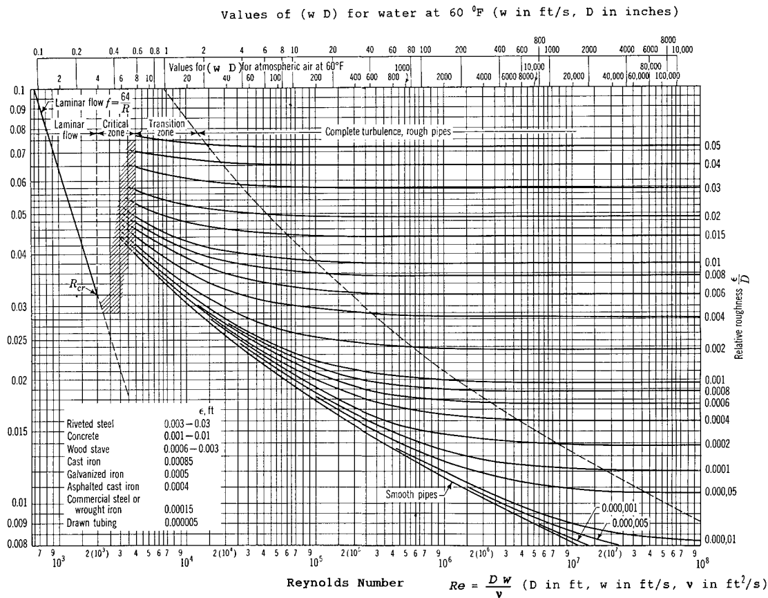
FIGURE B8.5 Moody diagram. (From Ref. 1.)
