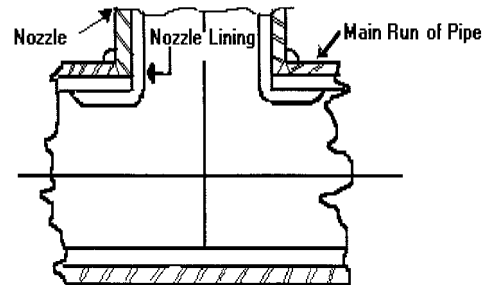
FIGURE B11.12 Rubber lining of nozzle or branch connection.
