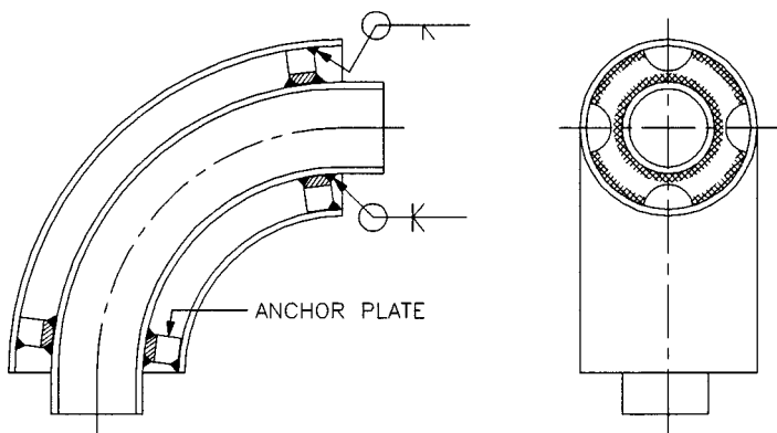
FIGURE B13.32 Restrained metallic elbow.
