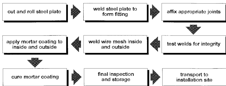
FIGURE A8.9 Fittings manufacturing process.
