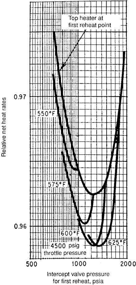
FIGURE C3.21 Relative performance for typical double-reheat units with various combinations of first-reheat intercept-valve pressure and final feedwater temperature. 27 (Courtesy of General Electric Co.)
