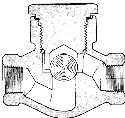
FIGURE A10.17 Ball check valve.
