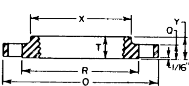
FIGURE A2.17 Typical loose flanges (threaded and slip-on).
