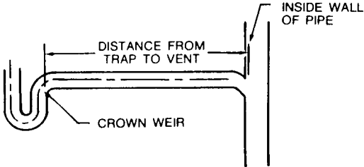
FIGURE C13.20 Trap arm.
