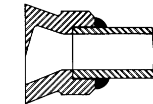
Socket detail for small welding and valve
